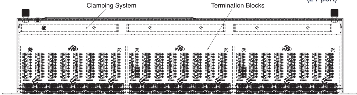
Front View (24 port)
