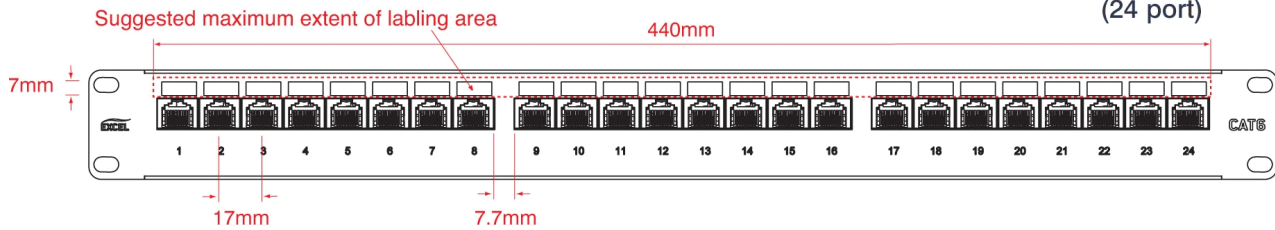
Front View (24 port)
